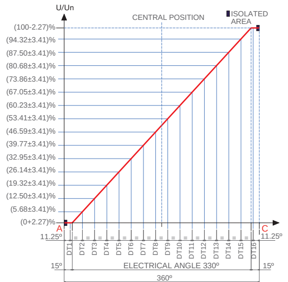
Electrical Taper Example: CSF14 HPL / HP
